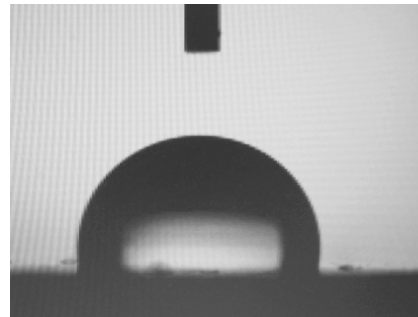
Figure 1. Contact angle measurement equipment(left) and profile of water drop
