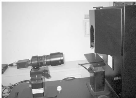
Figure 1. Contact angle measurement equipment(left) and profile of water drop
