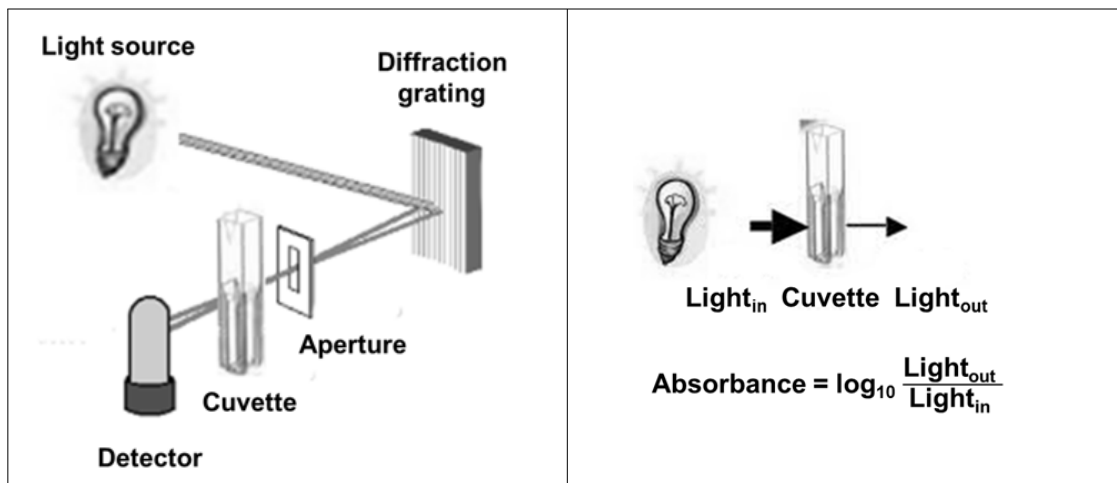
Figure 2. Absorbance measurement
