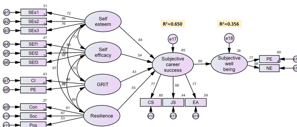
Fig. 2. Research model
