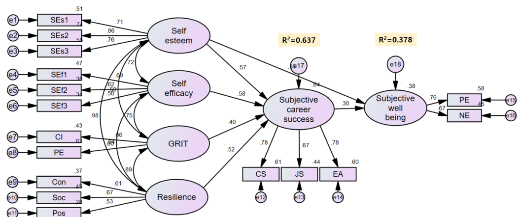
Fig. 3. Final model
