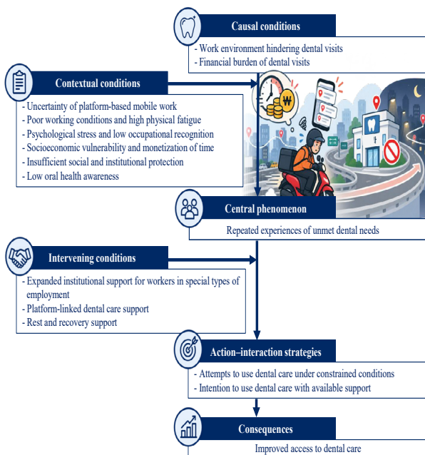
Fig. 1. Paradigm model.
